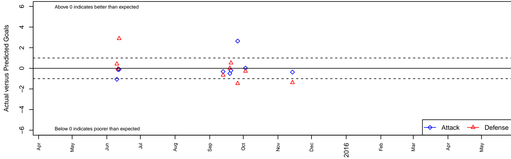
SFYS EFC Aftershocks G00 Dots are actual minus expected GF (blue circles) and GA (red triangles). Blue line is smoothed change in attack strength. Red is smoothed change in defense strength.
